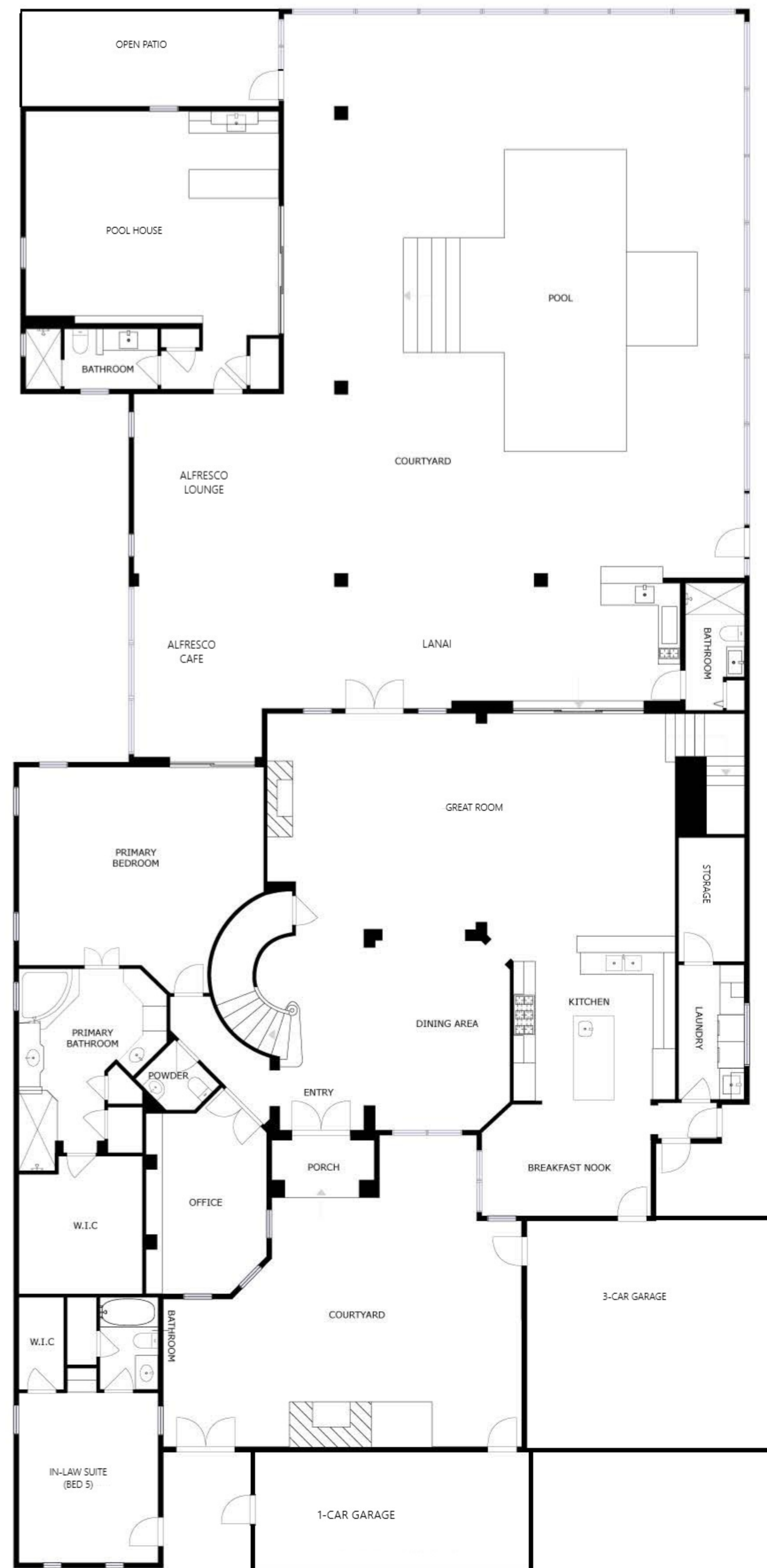
FLOOR 1
